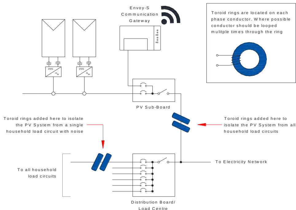
Figure 5: Toroid Ferrite Ring Installation Diagram
